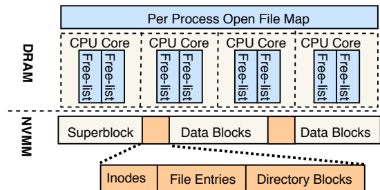
Figure 3: Simurgh Memory Layout
