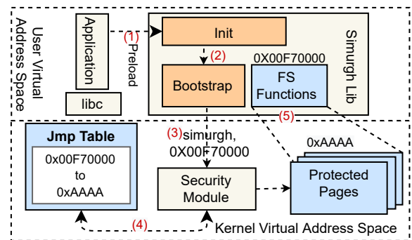
Figure 2: Security bootstrap of Simurgh
