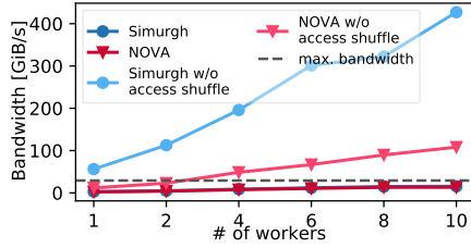
Figure 6: FxMark read (DRBL) performance
