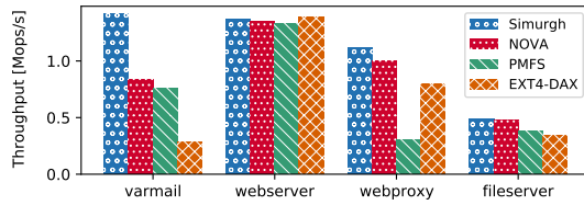
Figure 8: Throughput for Filebench workloads
