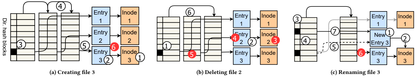
Figure 5: Shared directory metadata operations. The arrows depict the relative pointers to the metadata objects
